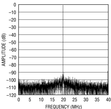
8192 Point FFT, f_{IN} = 140\text{MHz} , -1dB, 2V Range, 80Mps
